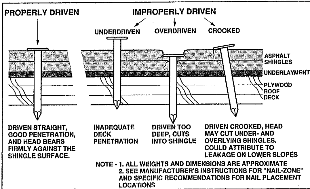
Figure 13 Example of fastener set for shingle nails.
